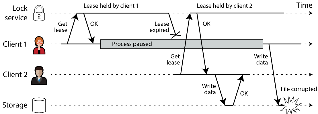
Figure 9-4. An incorrect implementation of a distributed lock: client 1 believes that it still has a valid lease, even though it has expired, and thus corrupts a file in storage
